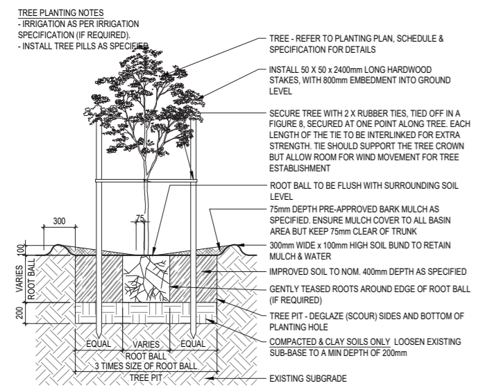
TYPICAL DETAIL - SEMI-ADVANCED TREE PLANTING
