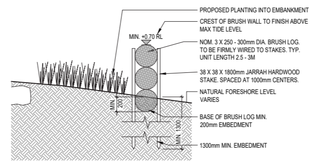
TYPICAL DETAIL - BRUSH WALLING
