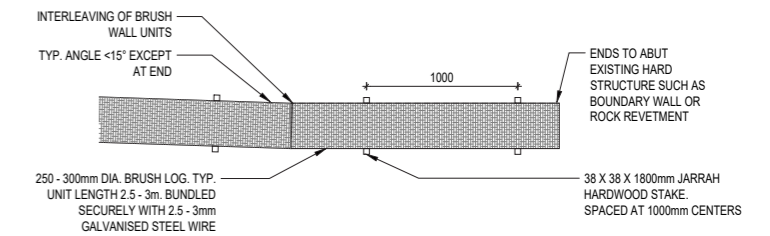
TYPICAL PLAN - BRUSH WALLING CONTINUOUS PLACEMENT
