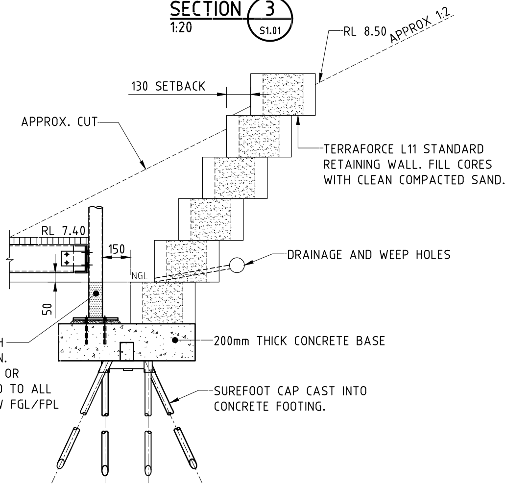
TYPICAL TERRAFORCE RETAINING WALL (TFRW2) 1:20
