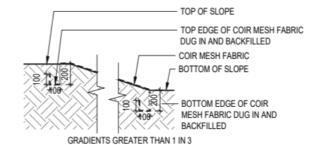
TYPICAL DETAIL - BIODEGRADABLE GEOTEXTILE FABRIC
