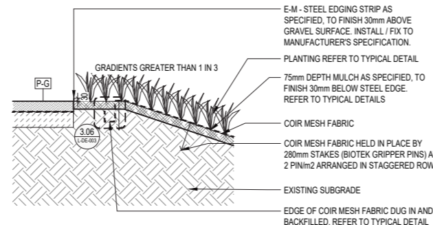
TYPICAL DETAIL - PLANTING ON SLOPE
