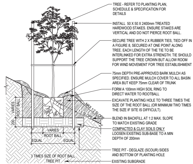
TYPICAL DETAIL - SEMI-ADVANCED TREE PLANTING ON EMBANKMENTS STEEPER THAN 1 IN 6
