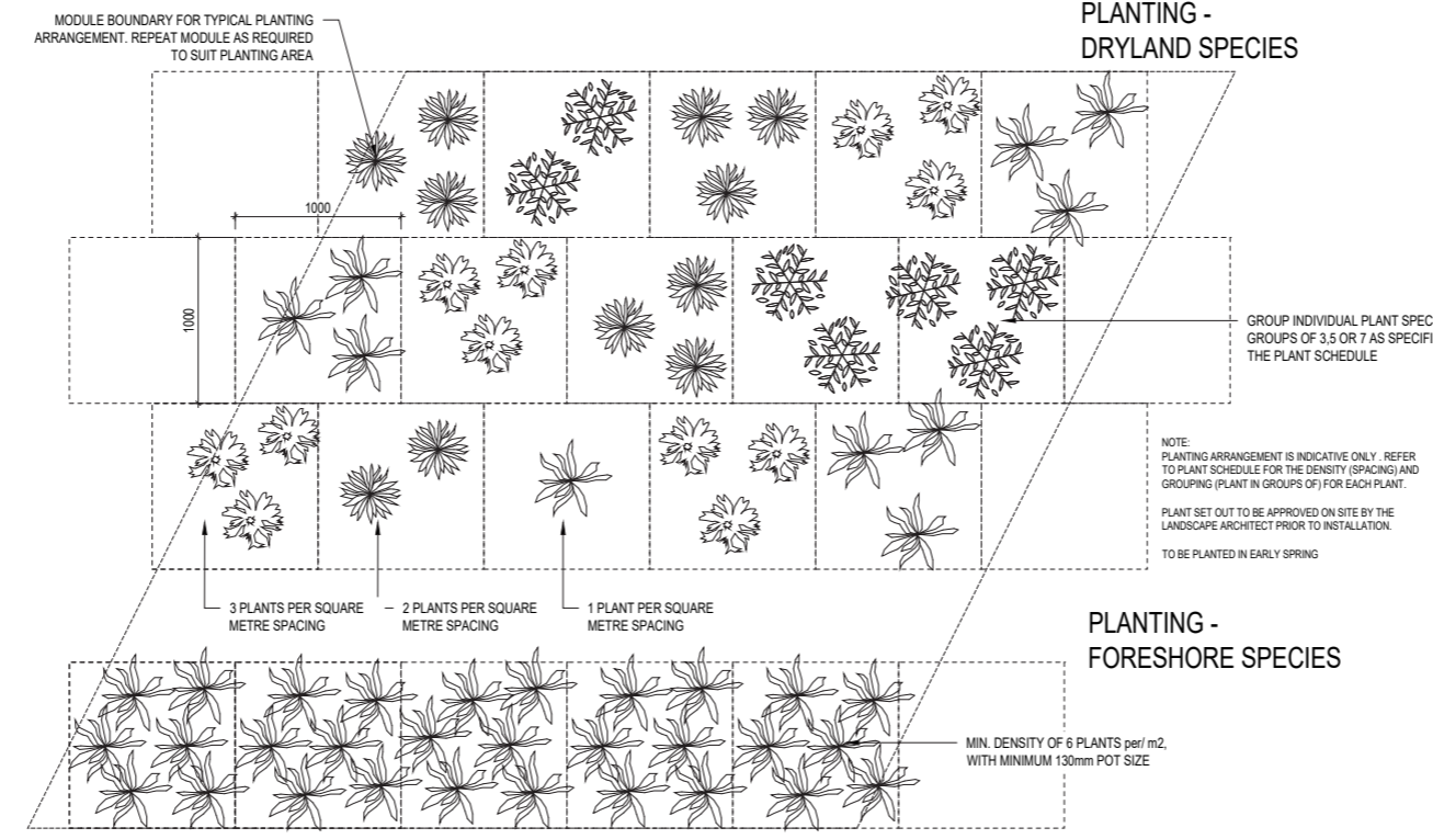
TYPICAL LAYOUT PLAN - PLANTING MIXES
