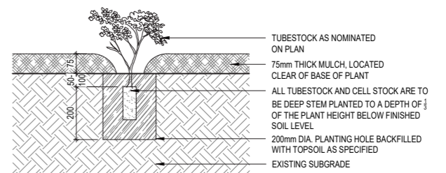
TYPICAL DETAIL - TUBESTOCK PLANTING METHOD
