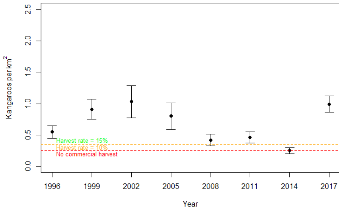
Fig. A3.3.2. Aerial survey density estimates with standard errors for red kangaroos in the South-East Zone from 1996 to 2017. All estimates use standard habitat correction factors (Table 2.2) and temperature corrections. Trigger point thresholds are included as horizontal lines. The South-East Zone is surveyed triennially.
